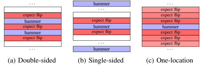
Fig. 2: Different hammering techniques as presented by [21].
