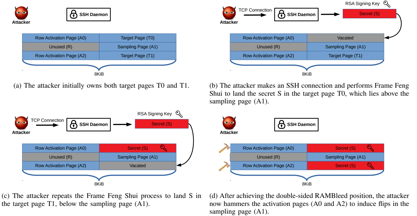
Fig. 5: Overview of our attack on OpenSSH
