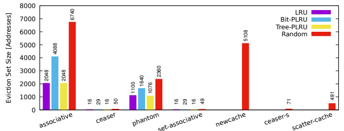
Fig. 9. Eviction set size for 2048-line caches and 90% eviction probability.
