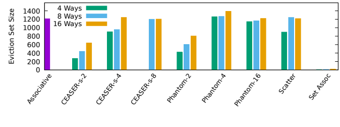
Fig. 13. Optimal eviction set sizes for different caches with 1024 lines
