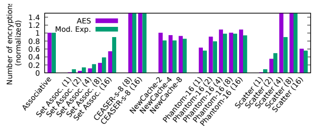
Fig. 10. Eviction-set attack: Number of encryptions required to break AES and modular exponentiation with random replacement. CEASER, CEASER-s-1, and Phantom-1, which show behavior similar to set associative caches, have been omitted from the figure. (Normalized to a random-replacement associative cache.)
