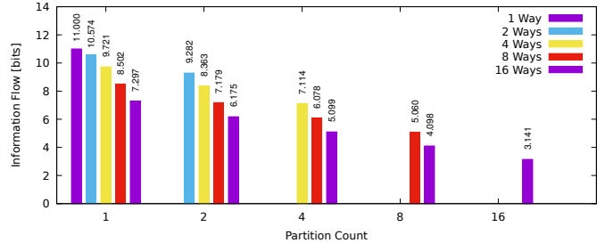
Fig. 3. REE for CEASER-S with 2048 lines depending on ways and partitions.
