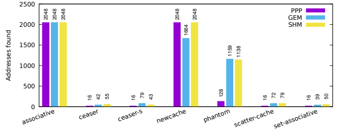
Fig. 7. Eviction set sizes found by eviction-set building techniques for different 2048-line caches.
