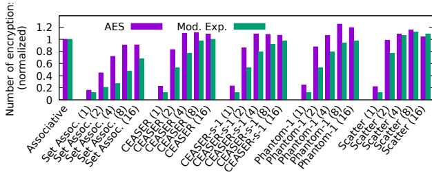
Fig. 11. Occupancy attack: Number of encryptions required to break AES and modular exponentiation with random replacement. CEASER-S-8, NewCache, and Phantom-16, which show behavior similar to fully associative caches, have been omitted from the figure. (Normalized to a random-replacement associative cache.)
