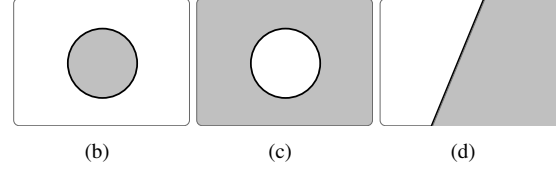
Figure 3. (a) A solid ball intersects the surface of a sphere at a spherical patch, which has a circular outline on the sphere. Under stereographic projection, a spherical patch is projected to become a circular patch. (b–d) The three types of circular patches: interior patch (this is the case in panel (a)), exterior patch (the spherical patch contains the pole; the “contents” of the spherical patch is projected outside of the circle), and half-plane (the pole lies on the circular outline of the spherical patch). See [11] for diagrams of projections that yield the two latter types.
