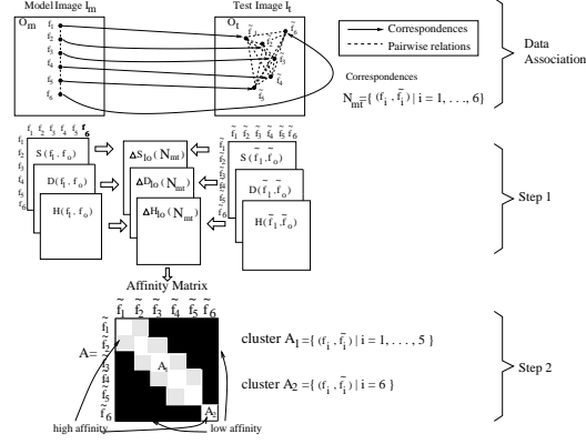
Fig. 1. Grouping based on pairwise relations. The data association consists of matching model and test features based solely on the similarity of their feature values (see Sec. III-A). Step 1 builds the pairwise similarity matrix as described in IV-A.1, and Step 2 comprises the clustering algorithm based on connected component analysis as defined in IV-A.2. Notice in the figure that correspondences 1 – 5 are semi-locally connected, while correspondence 6 is not. Therefore, two clusters are formed.
