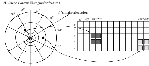
Fig. 2. Shape context of local feature f_1 . As in [4], we also use 5 bins for \log(\text{distance}) and 12 bins for relative orientation. Note that we modify the original shape context method as explained in Sec. IV-B.1.
