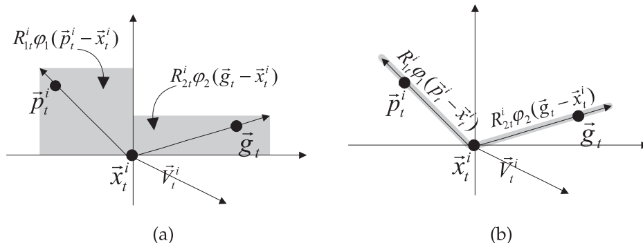
Figure 2: The gray areas are the areas in which \varphi_1 R_{1t}^i(\vec{p}_t^i - \vec{x}_t^i) and \varphi_2 R_{2t}^i(\vec{g}_t^i - \vec{x}_t^i) may be found, (a) SPSO, (b) LPSO.
