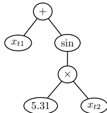
Fig. 1. GP representation of forecasting solution x_{t1} + \sin(5.31x_{t2})
