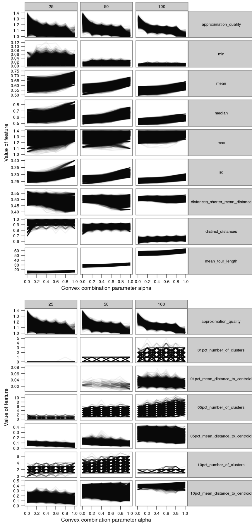
Figure 7: Distance features (top) and Cluster features (bottom): approximation quality and feature values for different \alpha levels of all conducted morphing experiments for Christofides.
