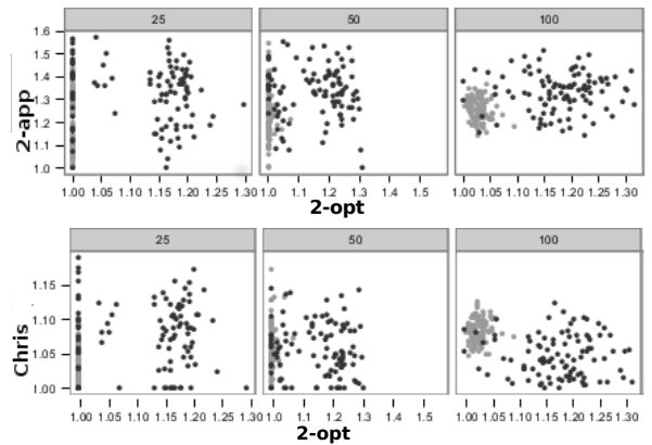
Figure 5: Performance of the 2-Approximation algorithm (top) and the Christofides algorithm (bottom) on the easy (grey) and hard (black) instances of 2-Opt algorithm.
