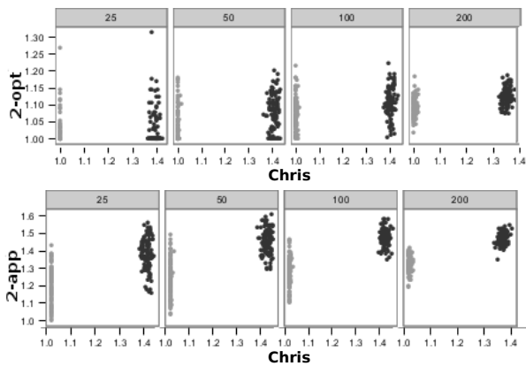
Figure 6: Performance of 2-Opt algorithm (top) and the 2-Approximation algorithm (bottom) on easy (grey) and hard (black) instances of Christofides algorithm.
