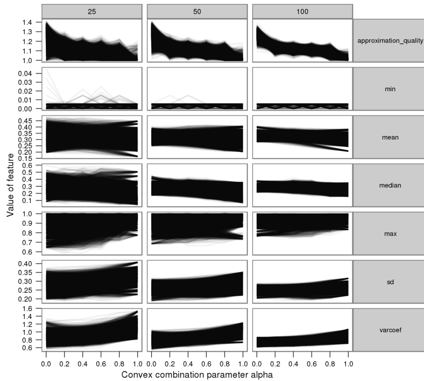
Figure 11: Nearest neighbour distance features: approximation quality and feature values for different \alpha levels of all conducted morphing experiments for Christofides.
