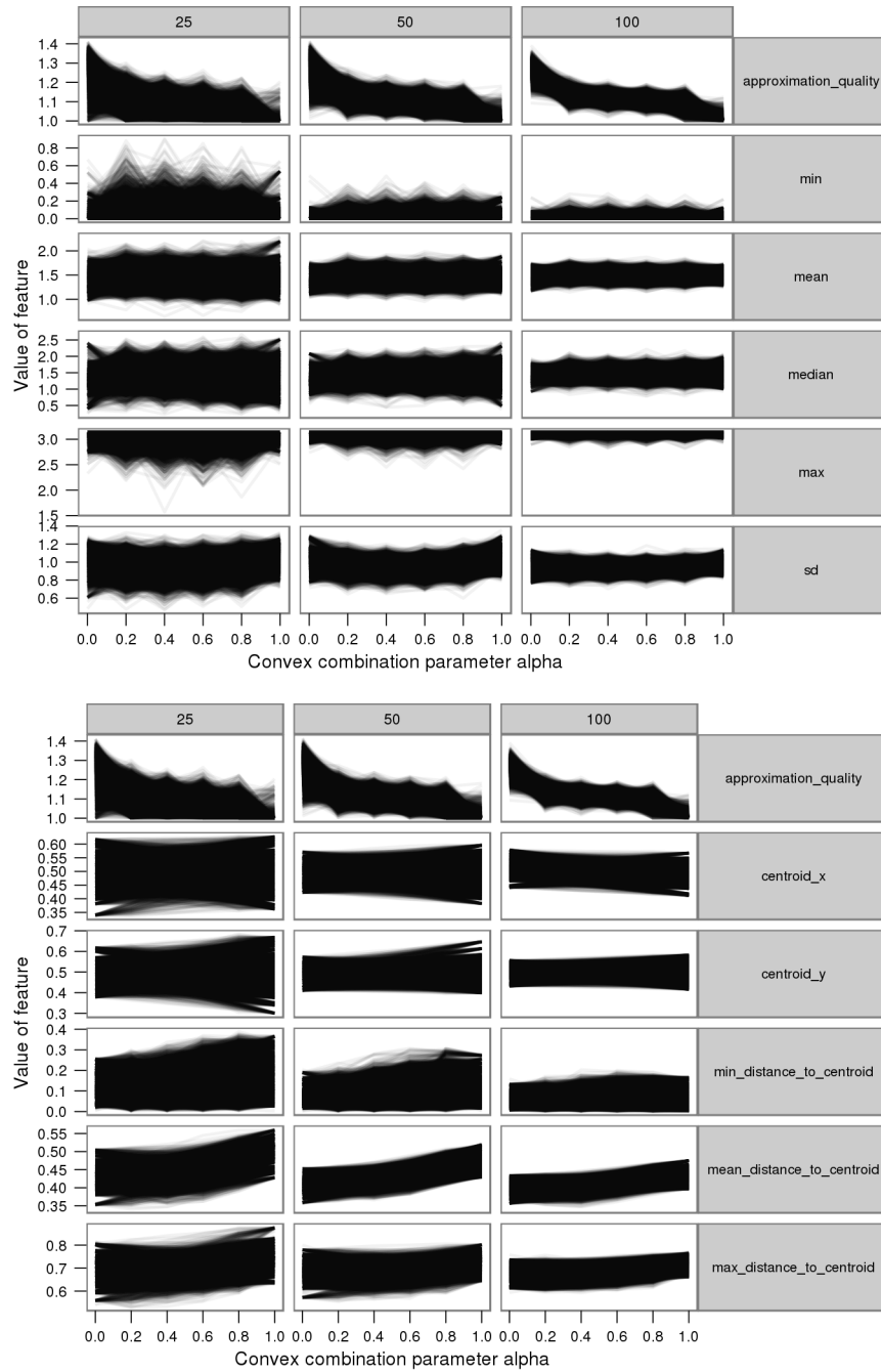
Figure 8: Angle (top) and Centroid Features (bottom): approximation quality and feature values for different \alpha levels of all conducted morphing experiments for Christofides.
