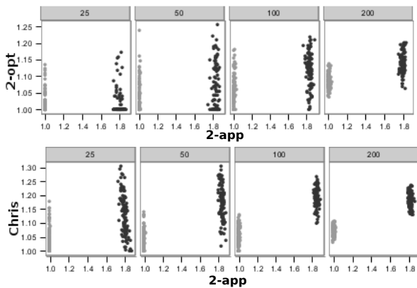
Figure 4: Performance of the 2-Opt algorithm (top) and Christofides algorithm (bottom) on the easy (grey) and hard (black) instances of the 2-Approximation algorithm.
