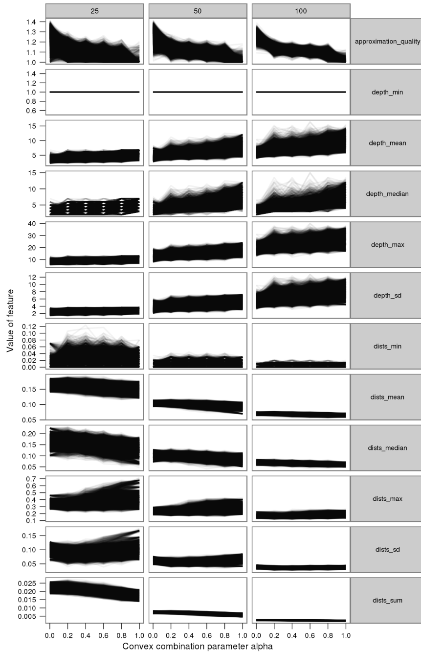
Figure 10: MST features: approximation quality and feature values for different \alpha levels of all conducted morphing experiments for Christofides.
