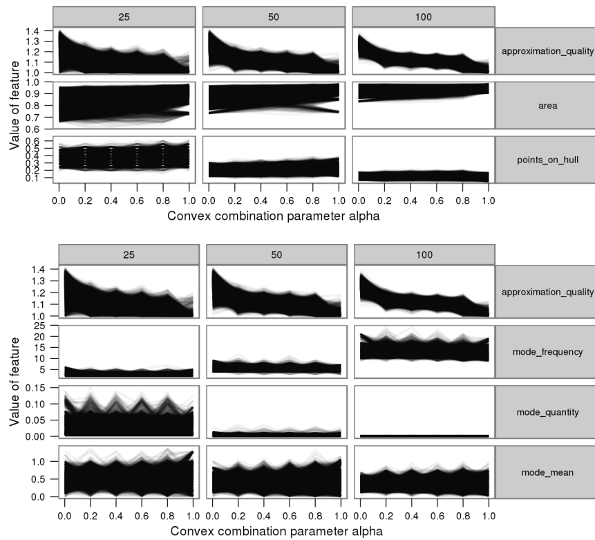
Figure 9: Convex Hull (top) and Mode (bottom) features: approximation quality and feature values for different \alpha levels of all conducted morphing experiments for Christofides.
