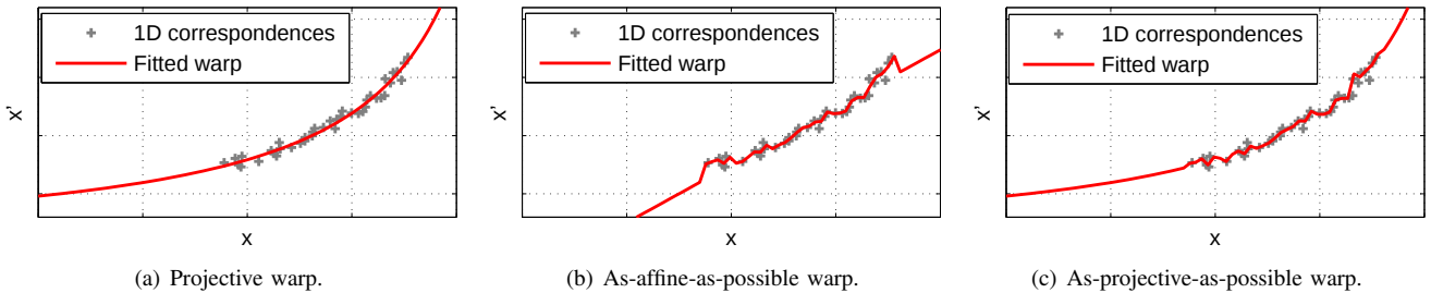
Fig. 2: To generate a 1D analogy of image stitching, a set of 1D correspondences \{\mathbf{x}_i, \mathbf{x}'_i\}_{i=1}^N are generated by projecting a 2D point cloud onto two 1D image “planes”. Here, the two views differ by a rotation and translation, and the data are not corrupted by noise. (a) A 1D projective warp, parametrised by a 2 \times 2 homography, is unable to model the local deviations of the data. Note that these deviations are caused purely by model inadequacy since there is no noise in the data. (b) An as-affine-as-possible warp, estimated based on [12], can interpolate the local deviations better, but fails to impose global projectivity. This causes incorrect extrapolation in regions without correspondences. (c) Our as-projective-as-possible warp interpolates the local deviations flexibly and extrapolates correctly following a global projective trend.
