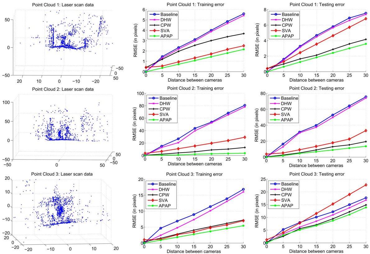
Fig. 5: Point cloud (left) and average RMSE on the training set (middle) and the testing set (right) as a function of inter-camera translational distance.
