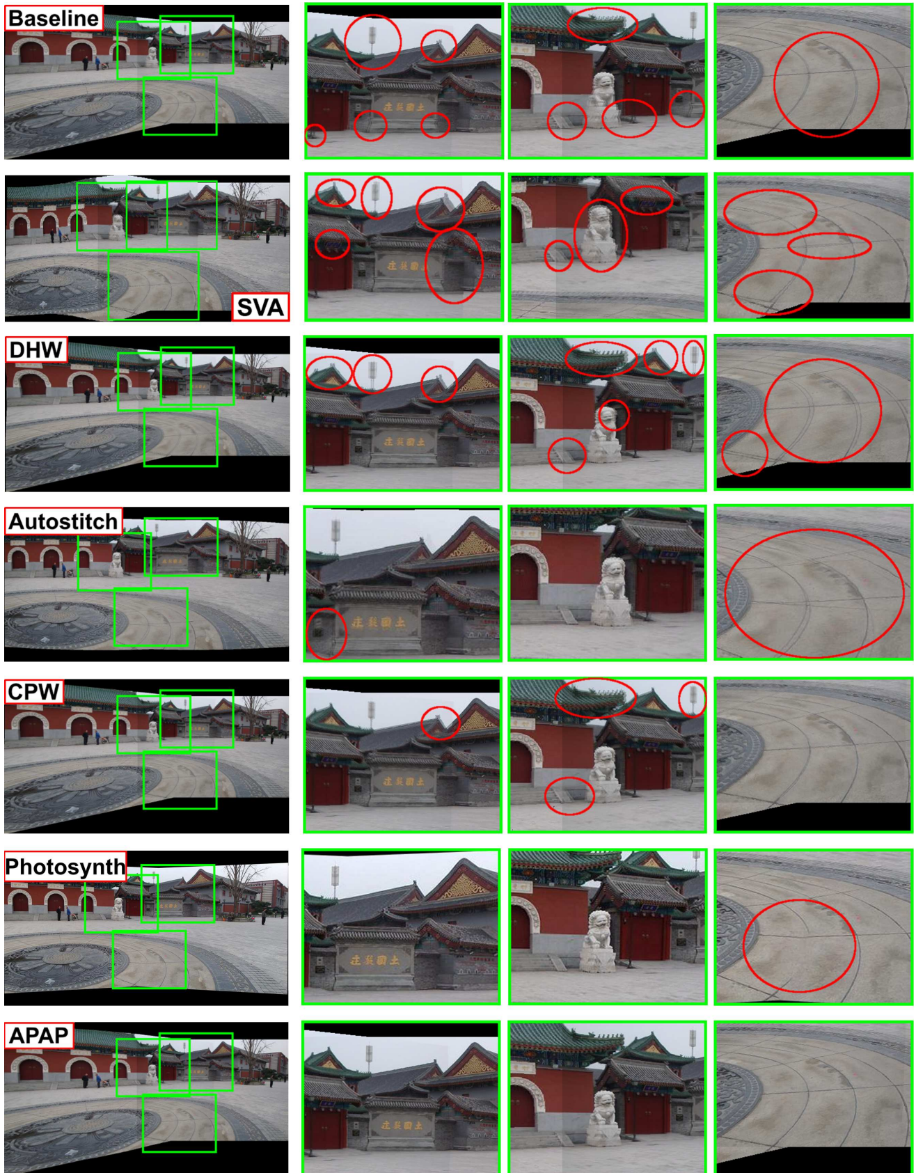
Fig. 7: Qualitative comparisons (best viewed on screen) on the temple image pair. Red circles highlight errors. List of abbreviations: SVA-Smoothly Varying Affine, DHW-Dual Homography Warps, CPW-Content Preserving Warps, APAP-As Projective As Possible Warps.
