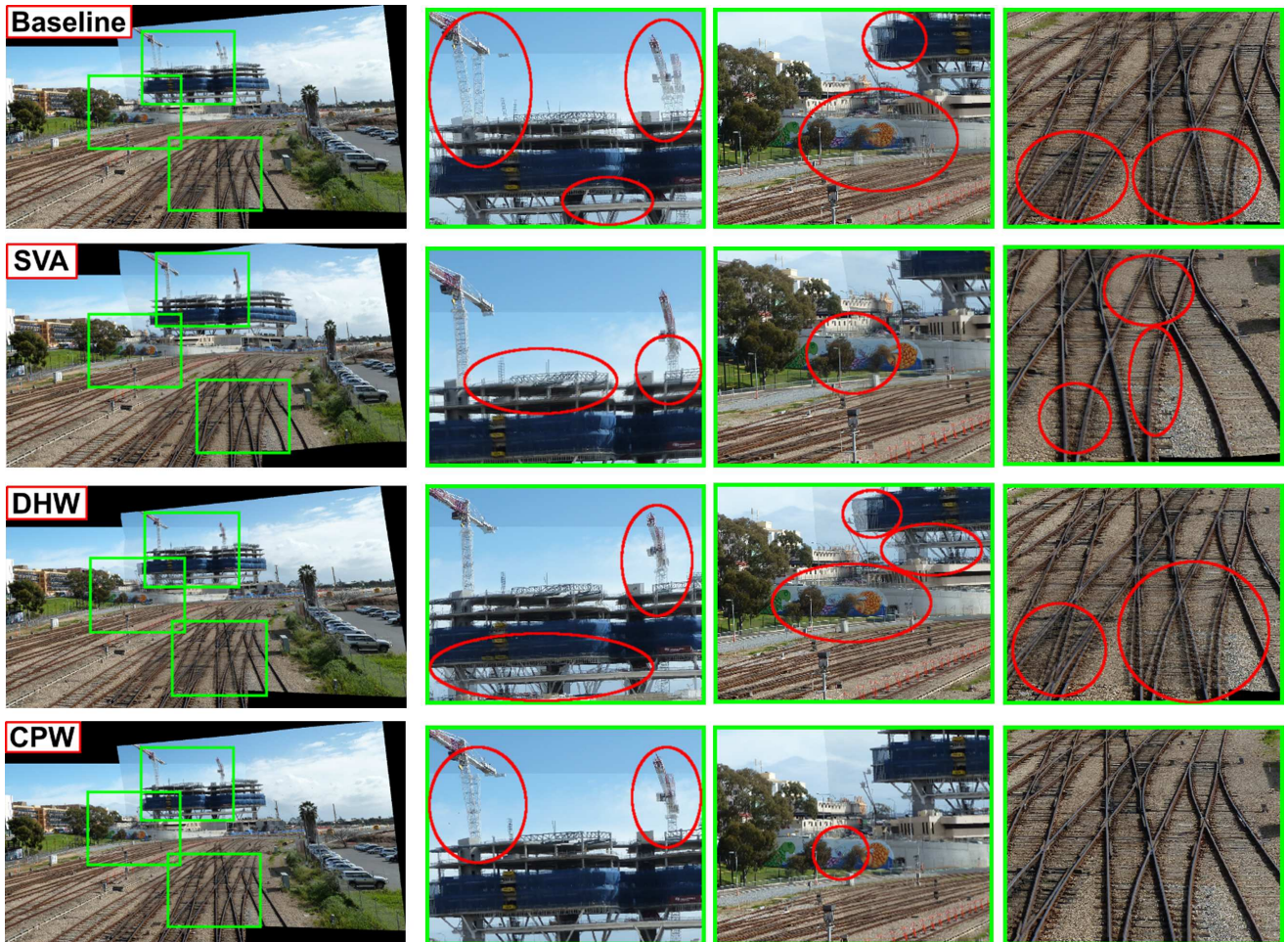
Fig. 6: Qualitative comparisons (best viewed on screen) on the railtracks image pair. Red circles highlight errors. List of abbreviations: SVA-Smoothly Varying Affine, DHW-Dual Homography Warps, CPW-Content Preserving Warps. Note that results for Autostitch, Photosynth and APAP are shown in Fig. 1.
