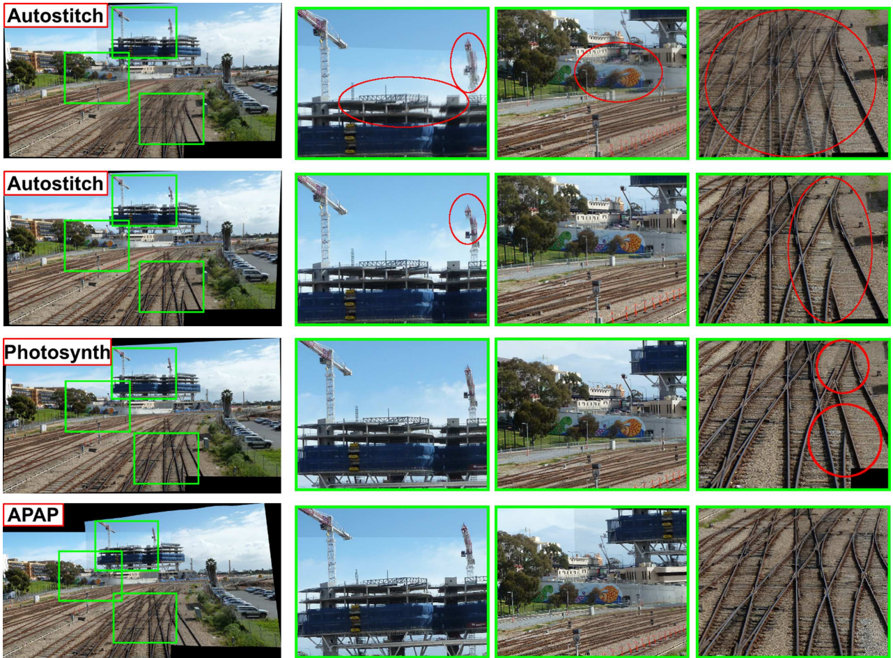
Fig. 1: Row 1: Raw alignment result from Autostitch [1] with significant ghosting. Rows 2 and 3: Final results (with advanced pixel compositing) from Autostitch and Photosynth, where glaring artifacts exist. Row 4: Raw alignment result using the proposed as-projective-as-possible method, which exhibits little noticeable ghosting.
