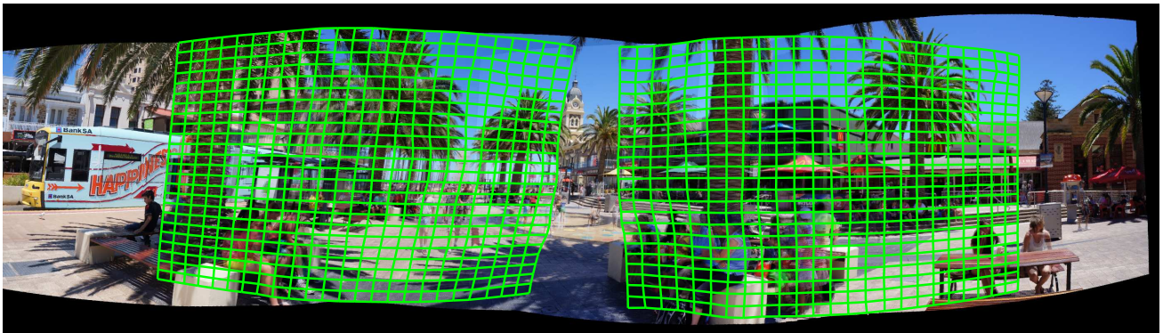
Fig. 8: Aligned images with transformed cells overlaid to visualize the multiple as-projective-as-possible warps refined using our novel bundle adjustment scheme (Sec. 4).
