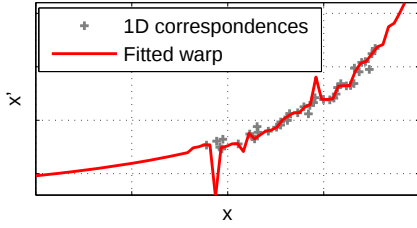
Fig. 3: Results from Moving DLT without regularisation for the 1D synthetic image stitching problem.
