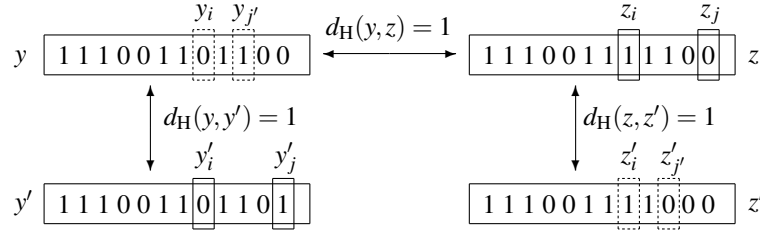
Fig. 1: An illustration of the proof of Lemma 10. Symbol d_H denotes the Hamming distance. If population \{y, z\} is updated, then the new set is either \{y, y'\} or \{z, z'\} , in which the two solutions maintain distance 1. The updates effectively swap the bits z_i, z_j or y_i, y_j , respectively.
